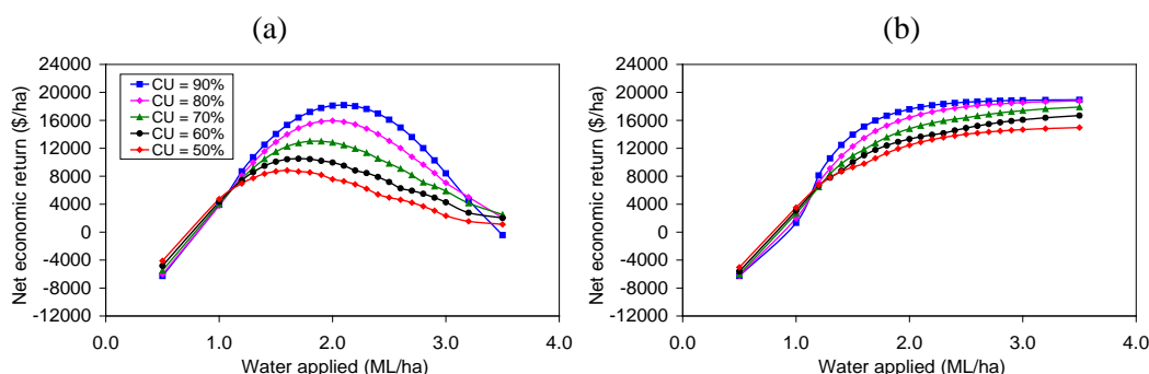
Figure 4 Effect of irrigation uniformity on the net economic return calculated using (a) quadratic and (b) exponential yield production functions from the winter trial
