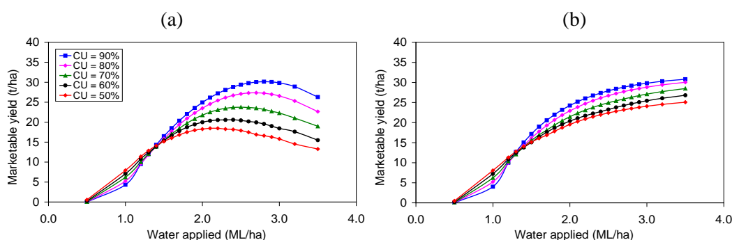
Figure 1 Effect of irrigation uniformity on the marketable yield of lettuce calculated using (a) quadratic and (b) exponential production functions from the autumn trial
